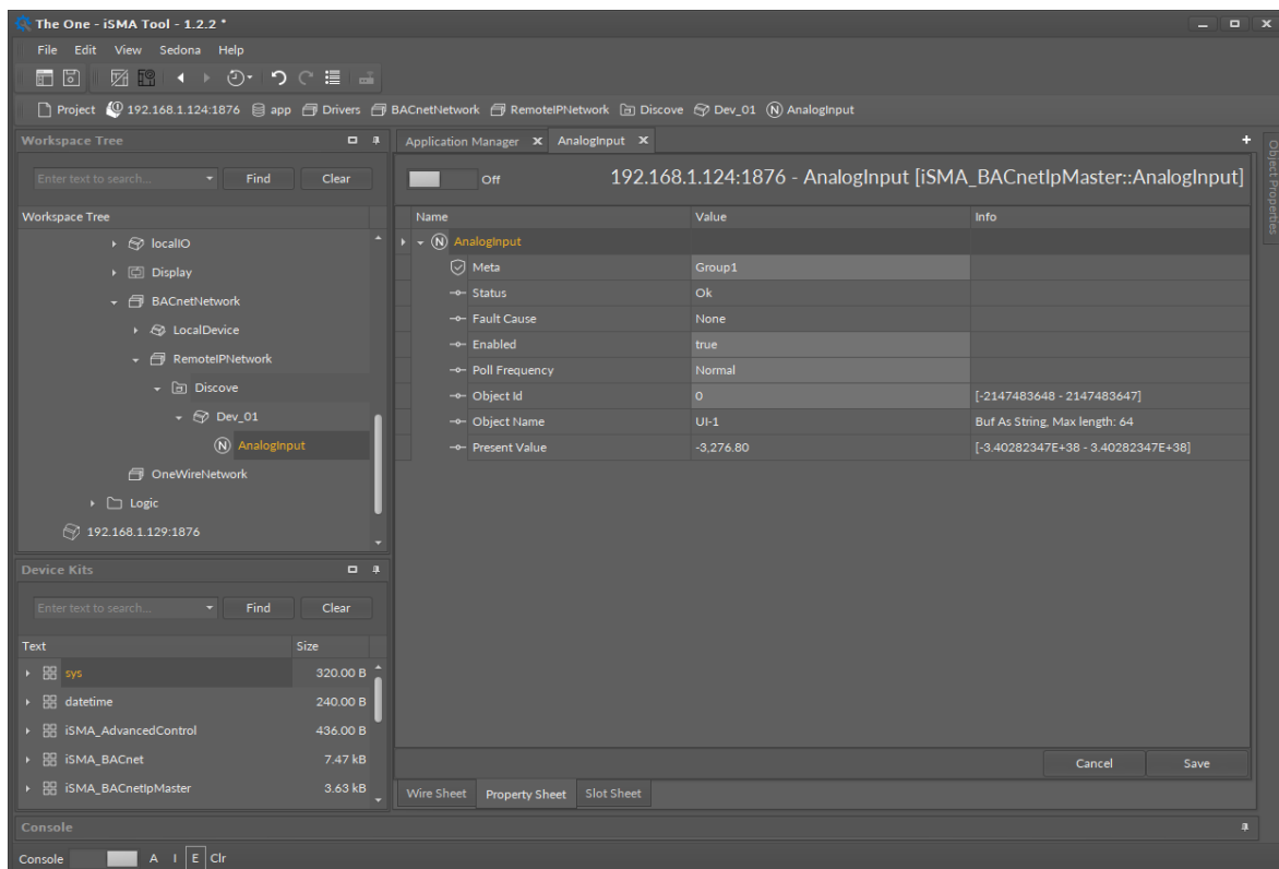
Figure 15. BACnet IP Analog Input Property Sheet view
