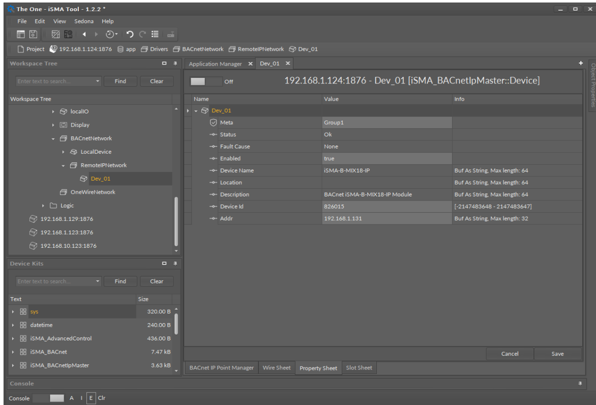
Figure 13. BACnet IP Master Device Property Sheet view
