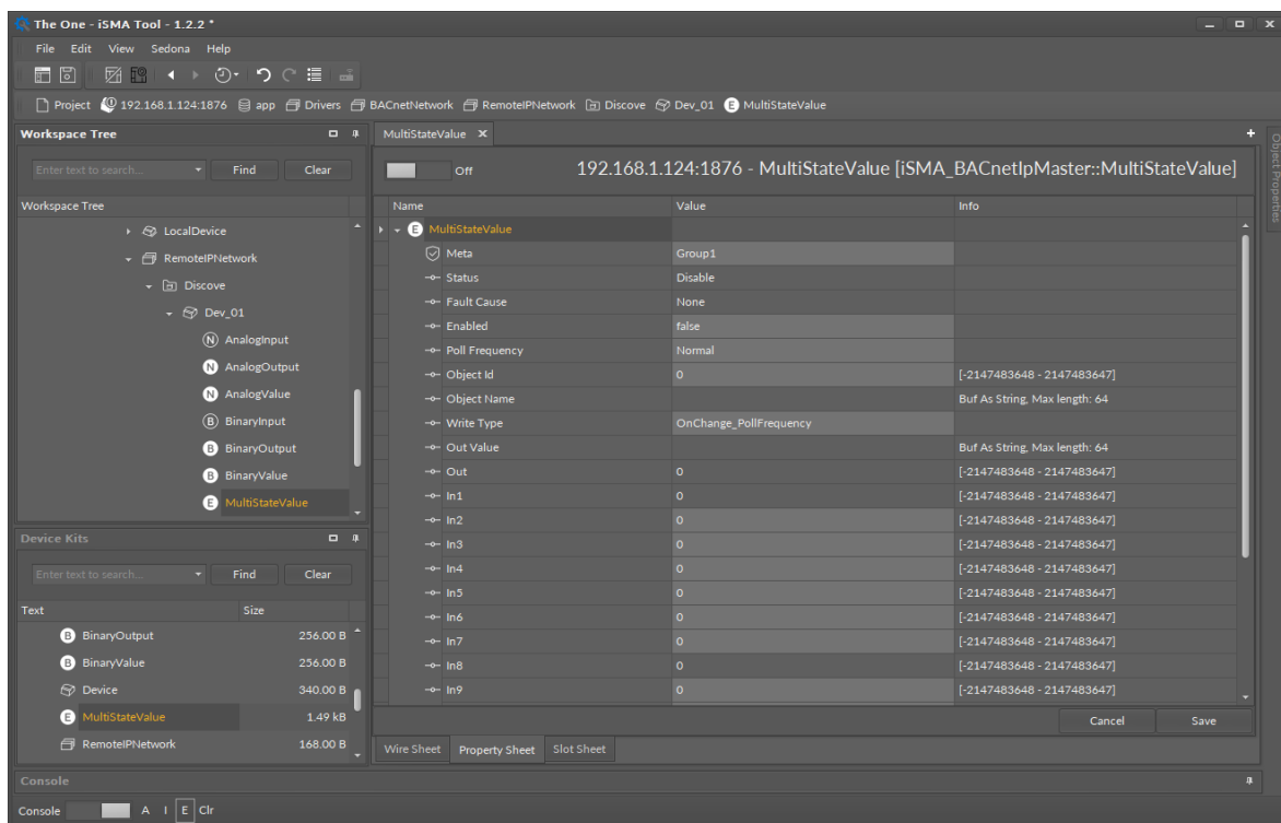
Figure 21. BACnet IP Multistate Value Property Sheet view
