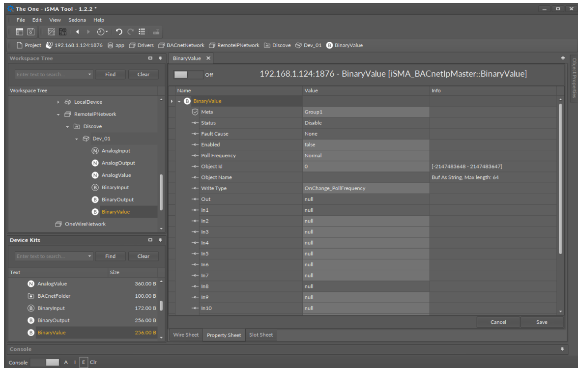
Figure 20. BACnet IP Binary Value Property Sheet view
