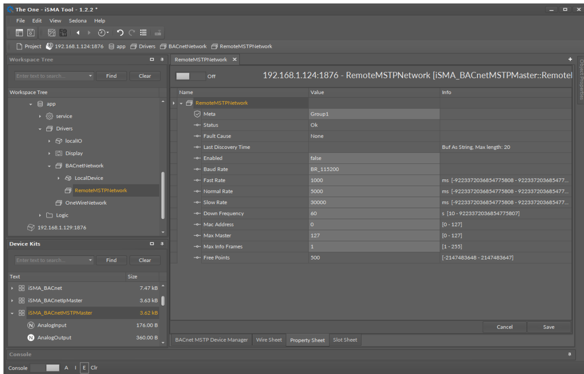
Figure 23. RemoteMSTPNetwork Property Sheet view
