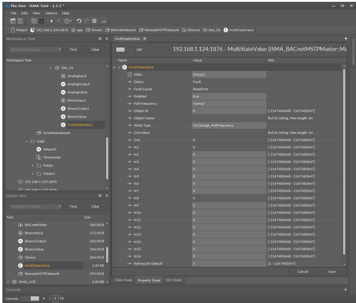
Figure 32. BACnet MSTP Multistate Value Property Sheet view
