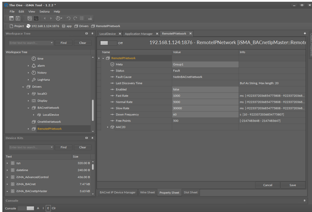
Figure 12. BACnet Remote IP Network Property Sheet view
