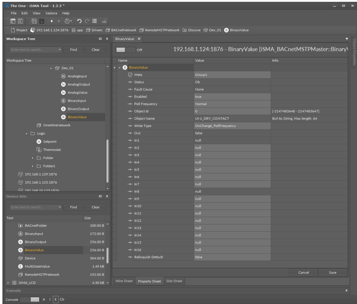
Figure 31. BACnet MSTP Binary Value Property Sheet view
