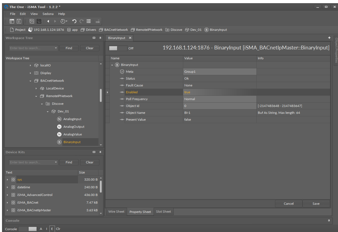
Figure 18. BACnet IP Binary Input Property Sheet view
