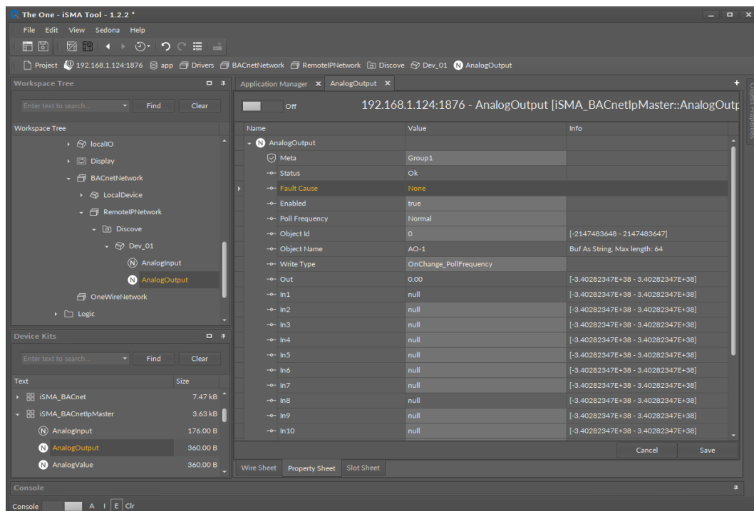
Figure 16. BACnet IP Analog Output Property Sheet view
