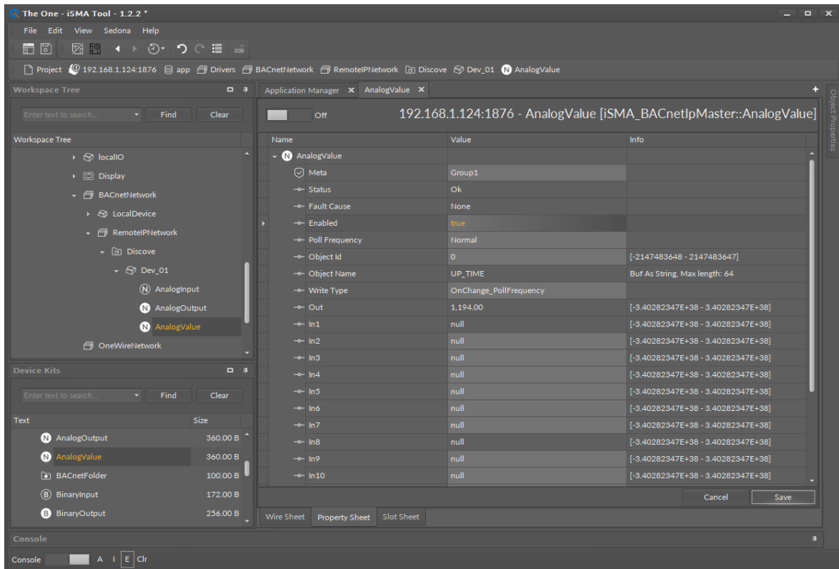
Figure 17. BACnet IP Analog Value Property Sheet view
