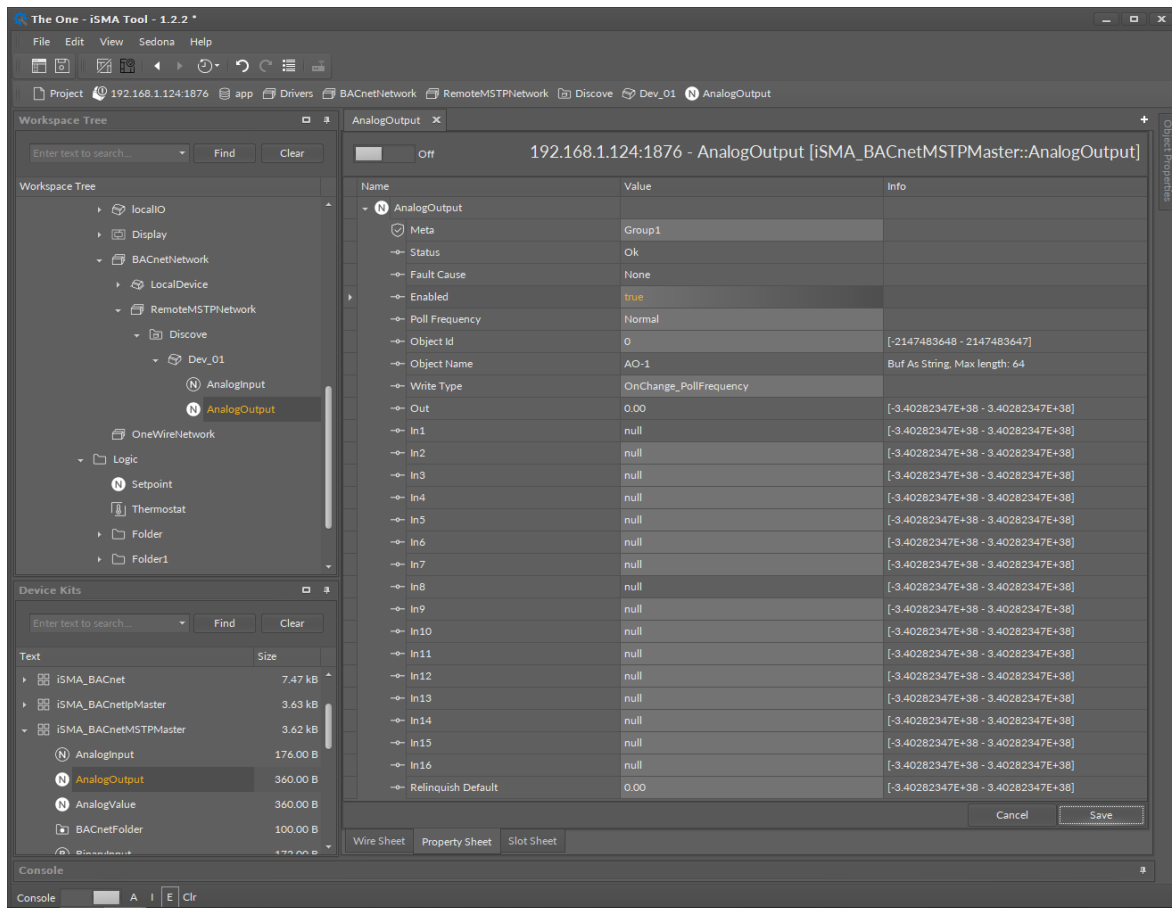
Figure 27. BACnet MSTP Analog Output Property Sheet view
