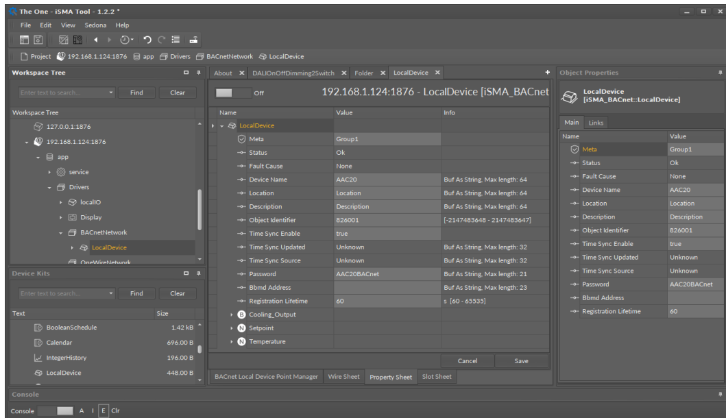
Figure 3. The BACnet Local Device property Sheet view
